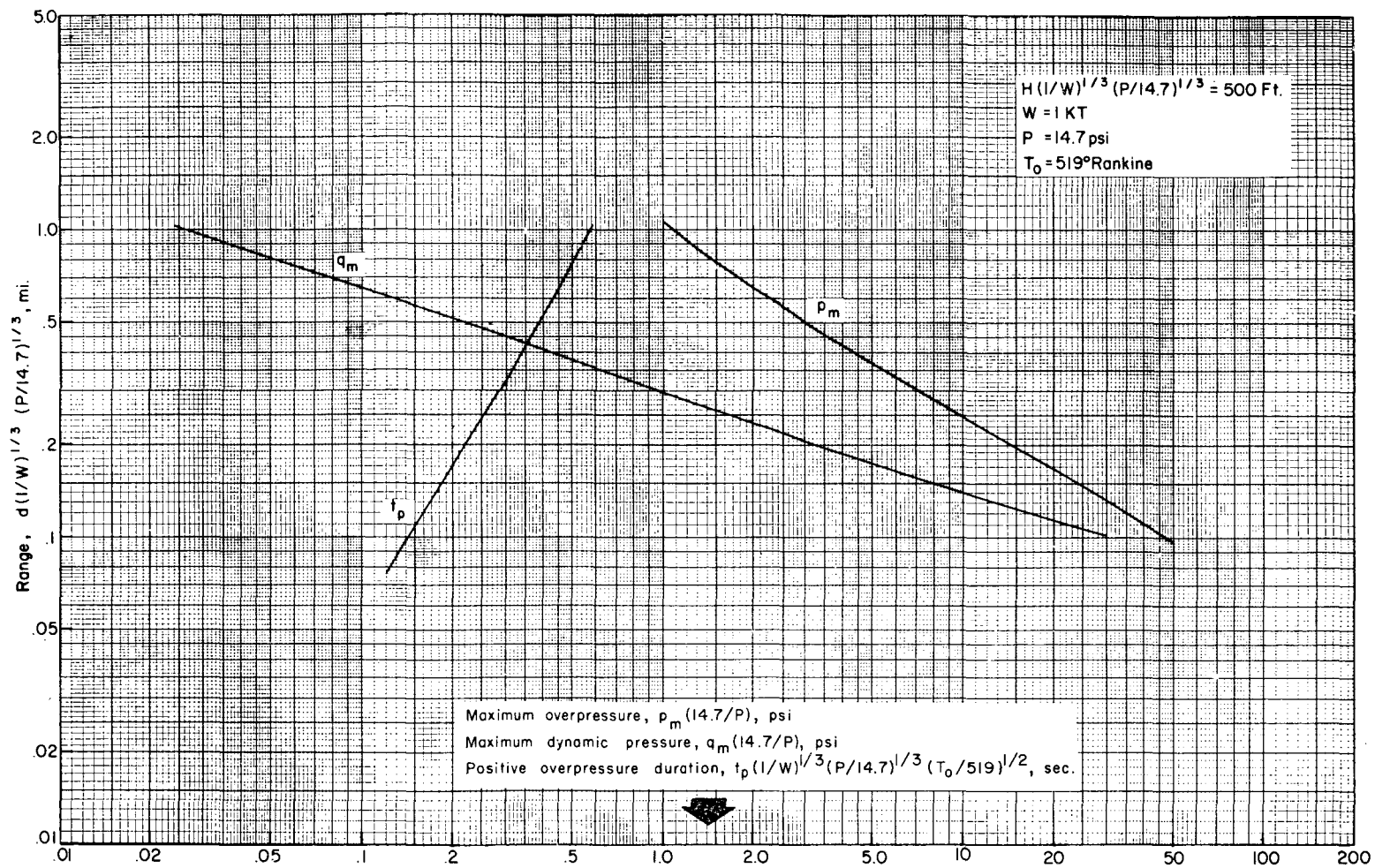
Fig. 2.6—Scaled blast parameters for a scaled height of burst of 500 ft as a function of scaled range. These are plots of Eqs. 2.42, 2.44, and 2.46 given in Table 2.6.
